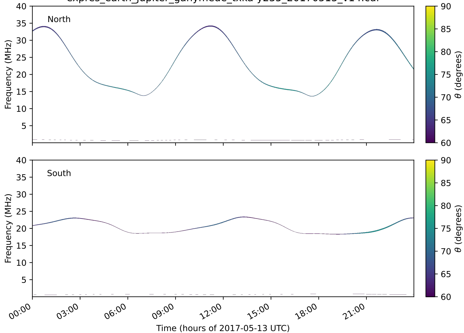
expres_earth_jupiter_ganymede_txka-y235_20170513_v14.cdf
