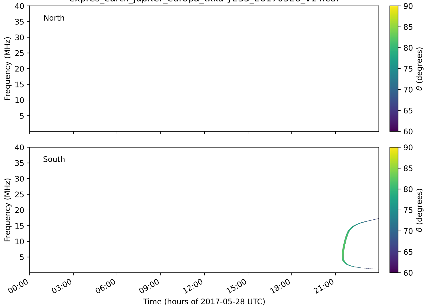
expres_earth_jupiter_europa_txka-y235_20170528_v14.cdf
