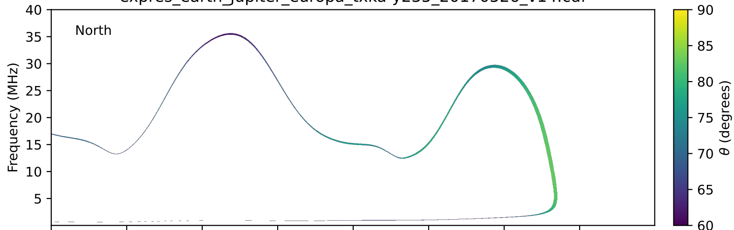
expres_earth_jupiter_europa_txka-y235_20170526_v14.cdf
