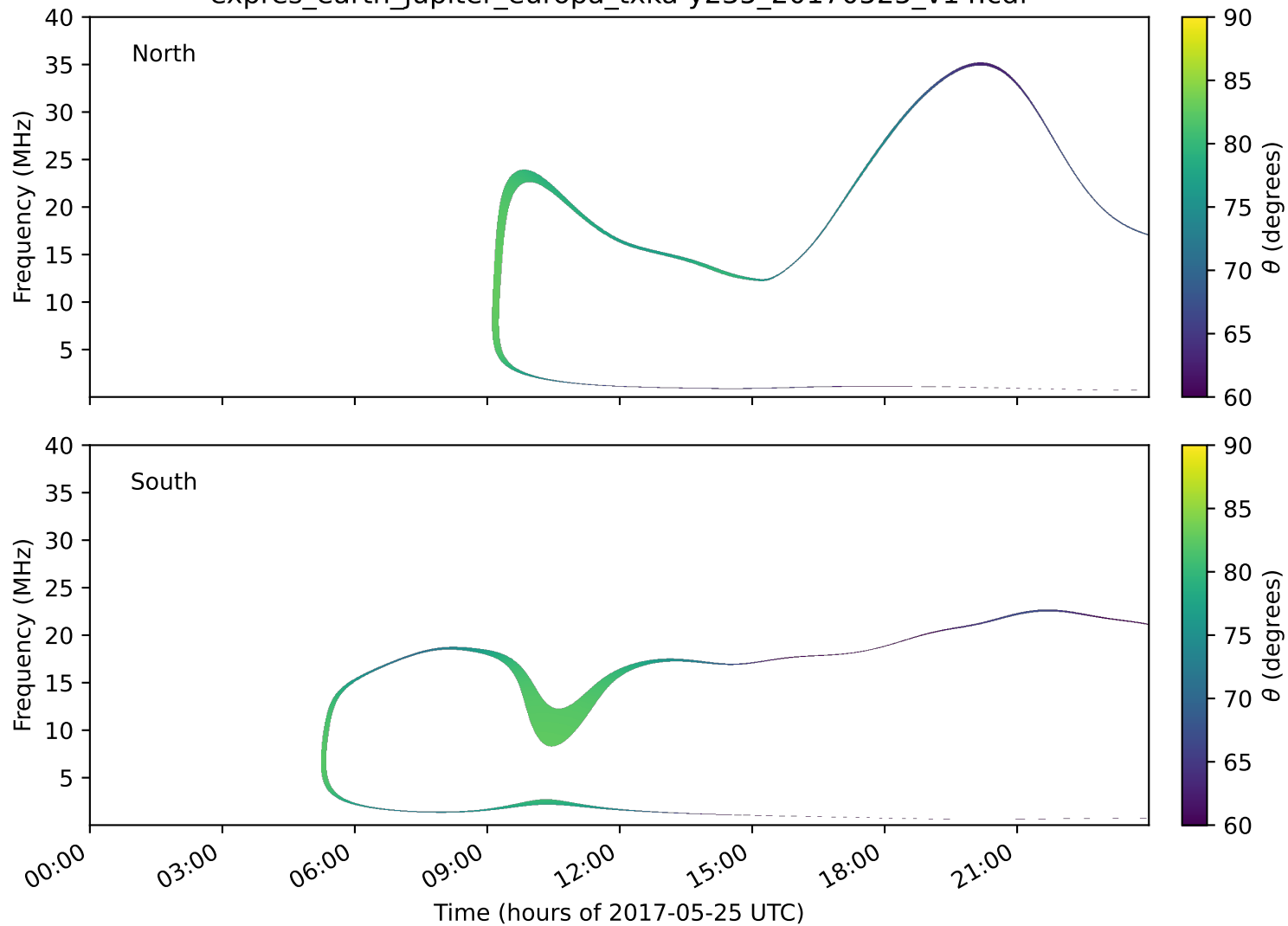
expres_earth_jupiter_europa_txka-y235_20170525_v14.cdf
