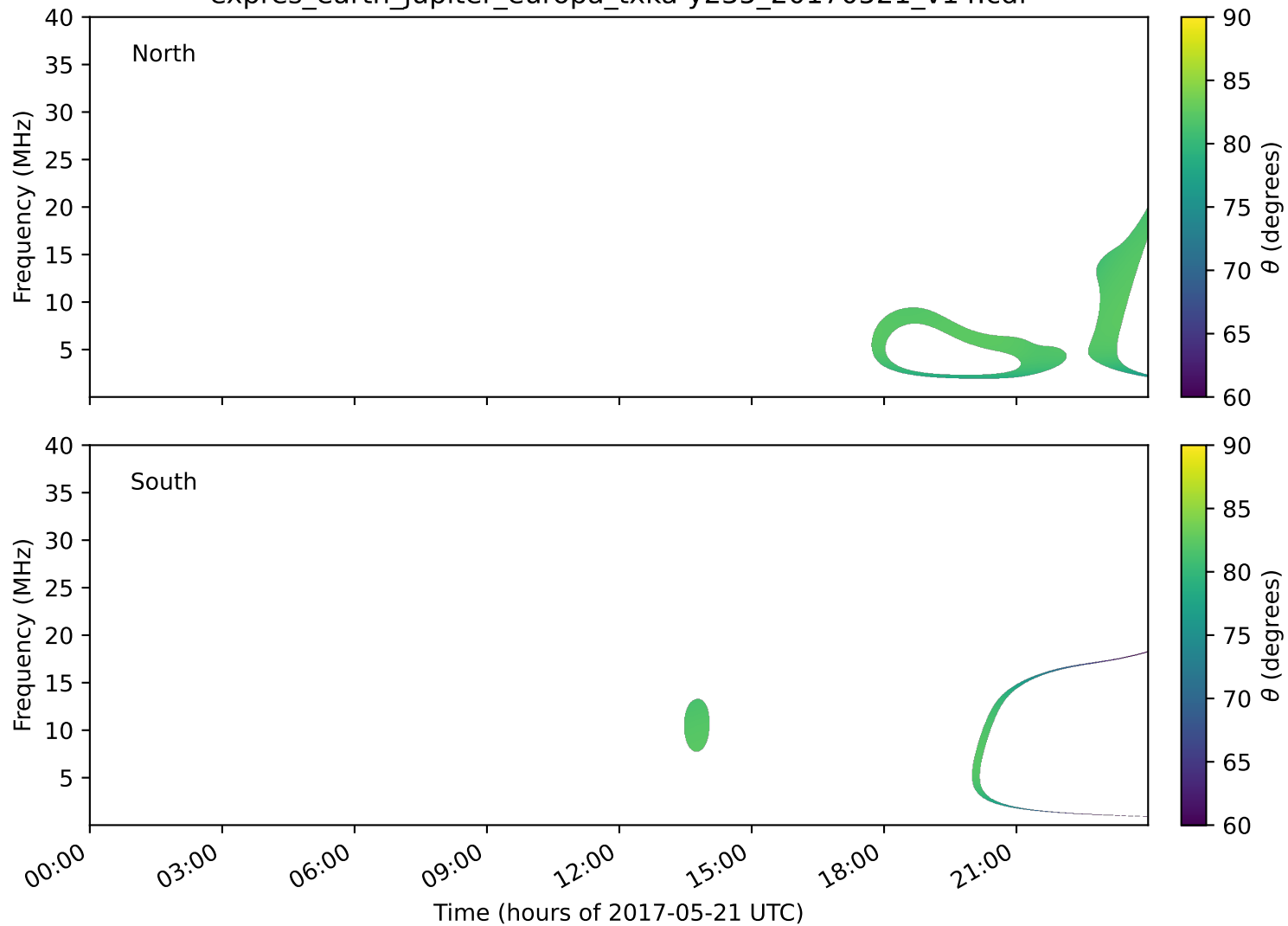
expres_earth_jupiter_europa_txka-y235_20170521_v14.cdf
