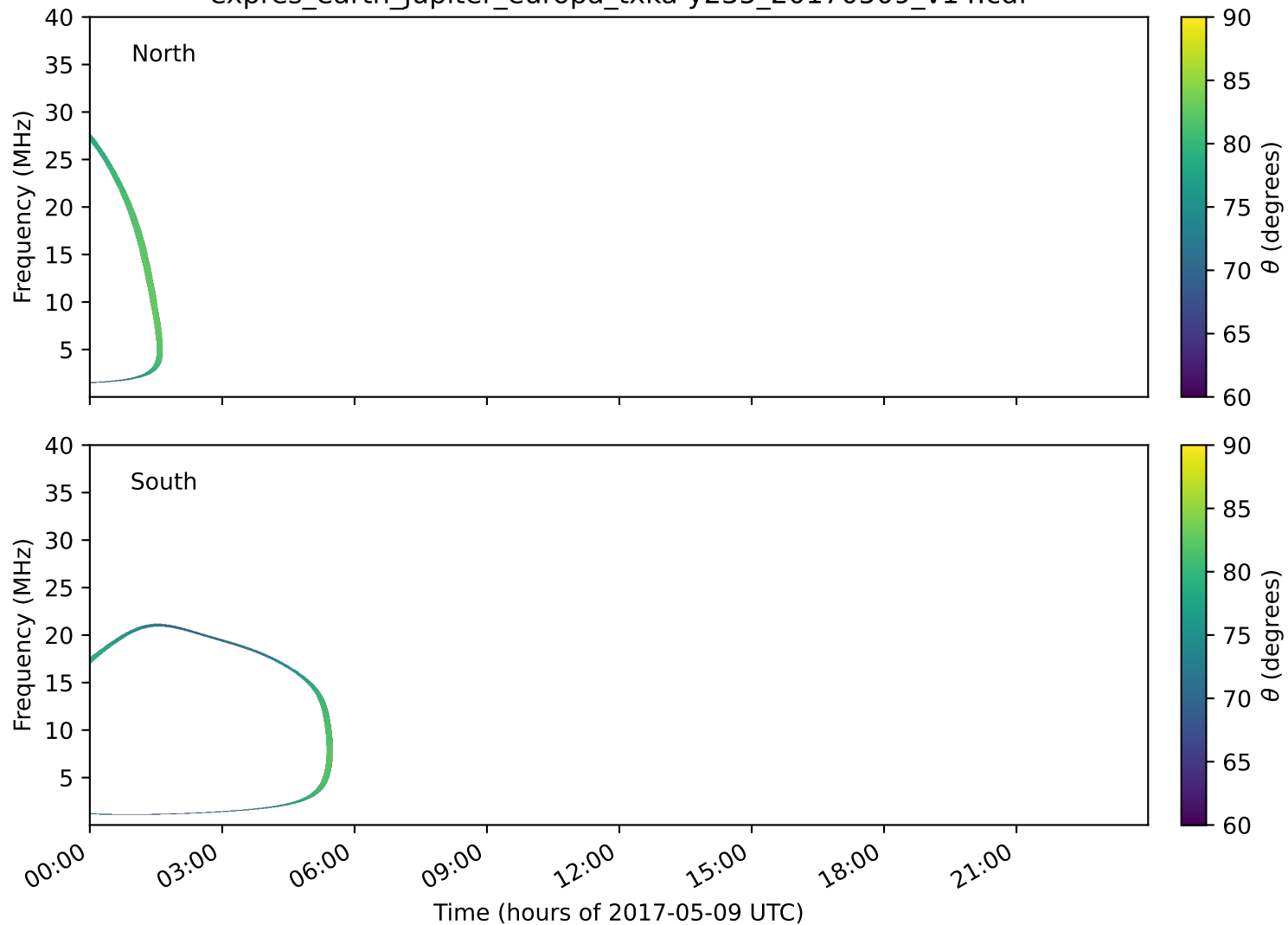
expres_earth_jupiter_europa_txka-y235_20170509_v14.cdf
