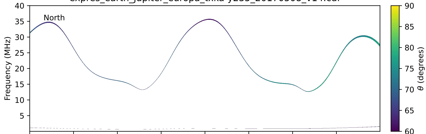
expres_earth_jupiter_europa_txka-y235_20170508_v14.cdf
