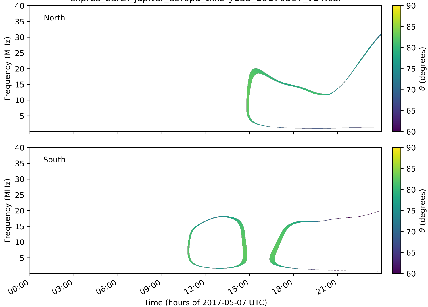
expres_earth_jupiter_europa_txka-y235_20170507_v14.cdf
