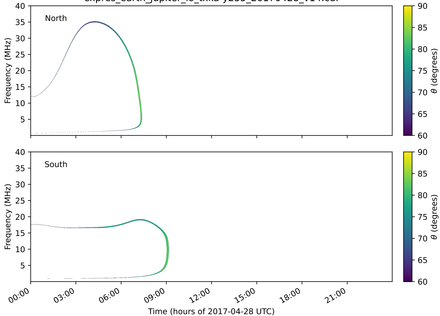
expres_earth_jupiter_io_txka-y235_20170428_v14.cdf
