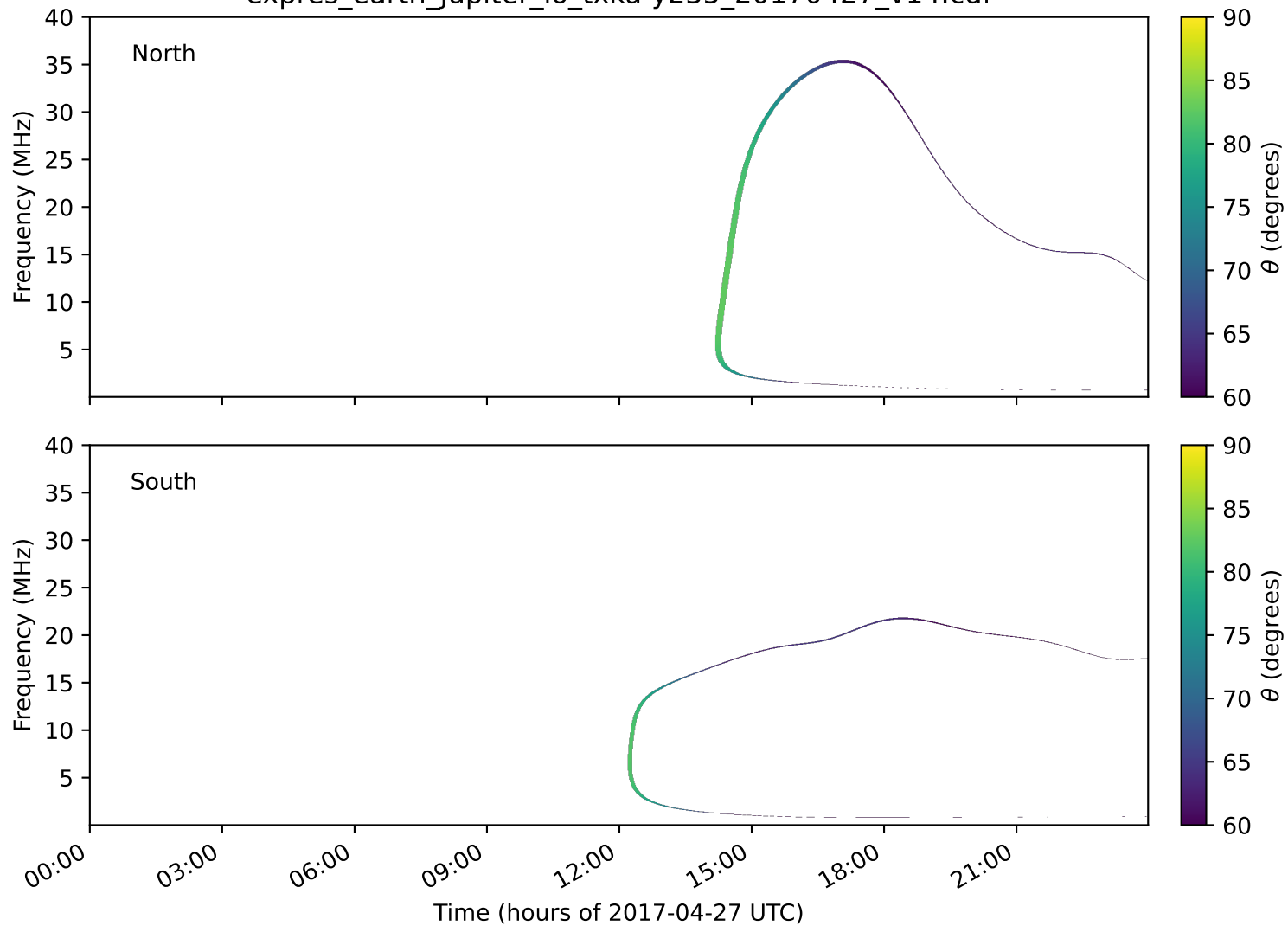
expres_earth_jupiter_io_txka-y235_20170427_v14.cdf
