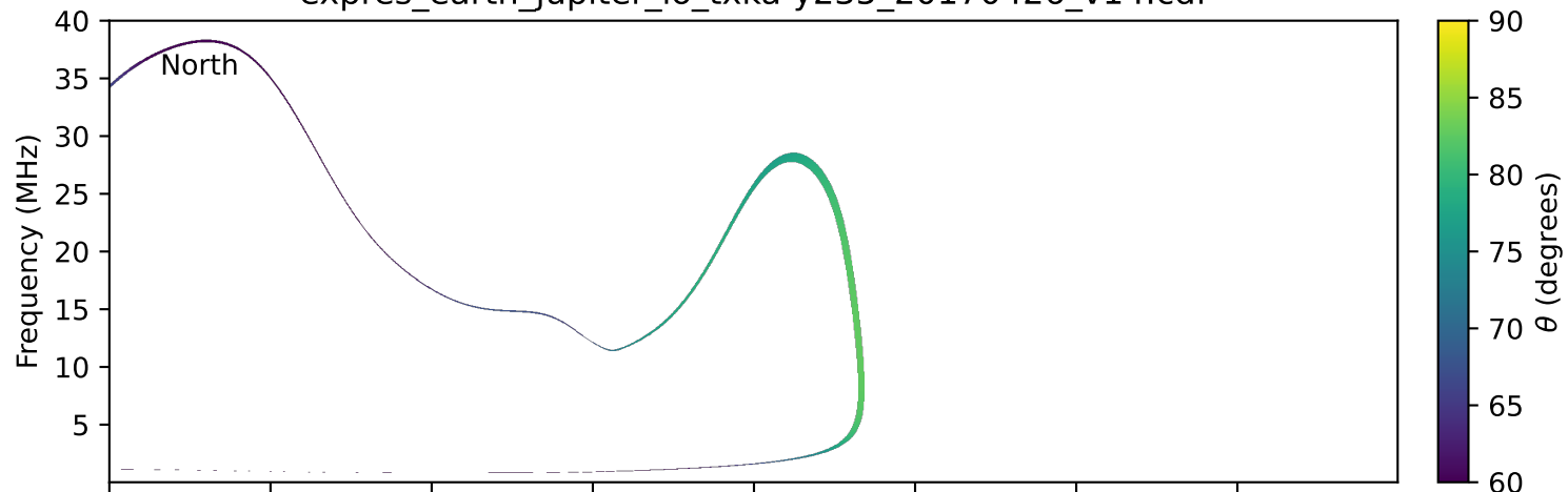
expres_earth_jupiter_io_txka-y235_20170426_v14.cdf
