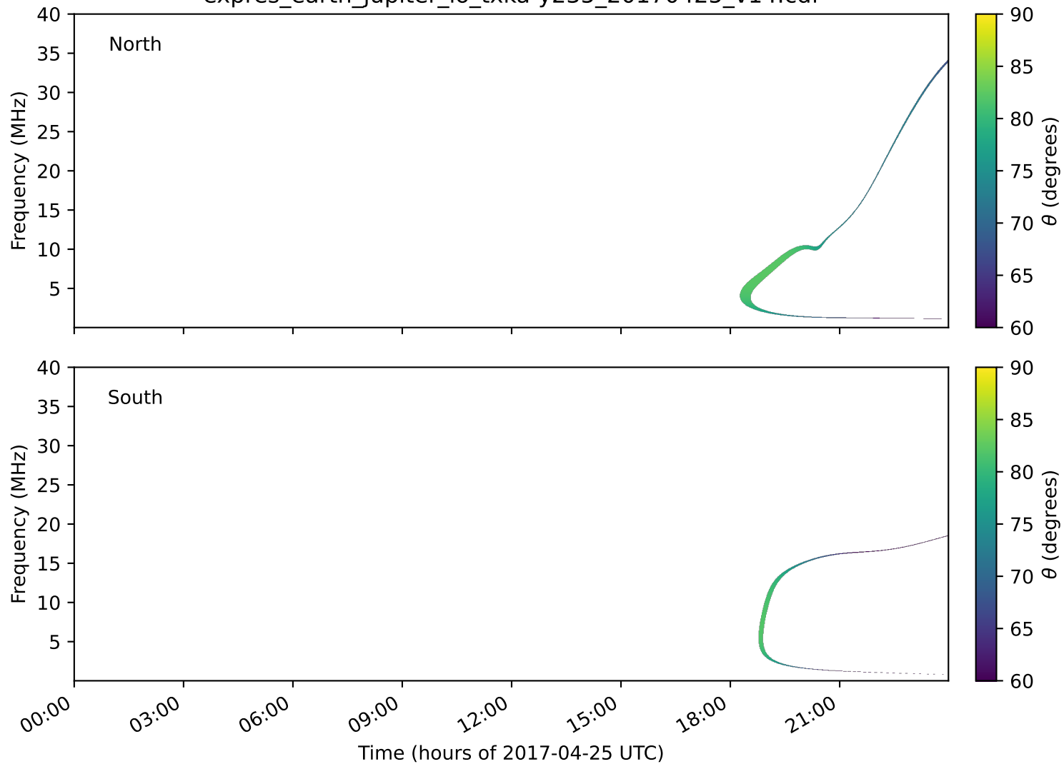
expres_earth_jupiter_io_txka-y235_20170425_v14.cdf
