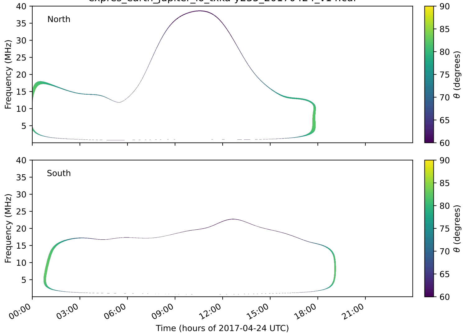
expres_earth_jupiter_io_txka-y235_20170424_v14.cdf
