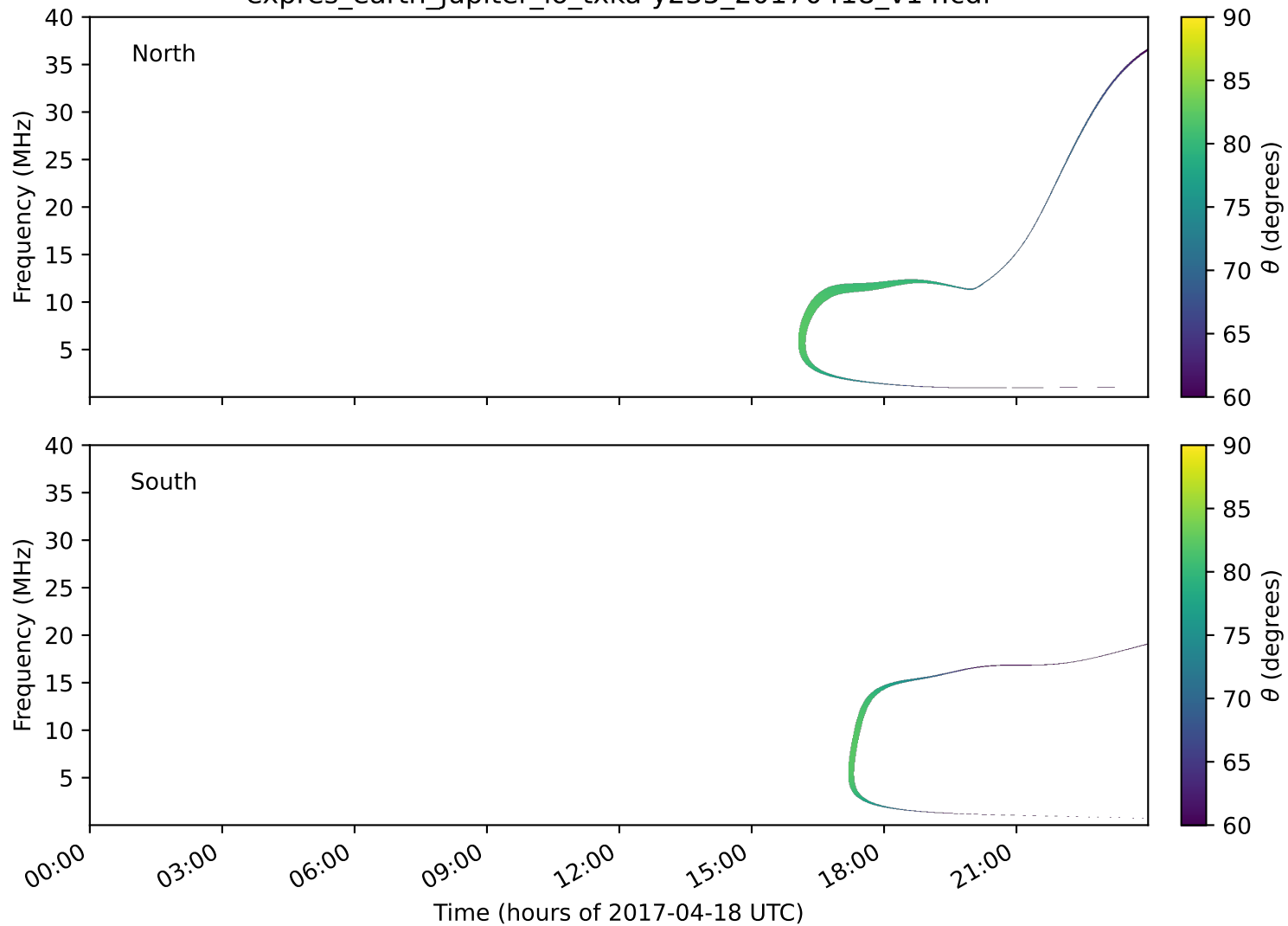
expres_earth_jupiter_io_txka-y235_20170418_v14.cdf
