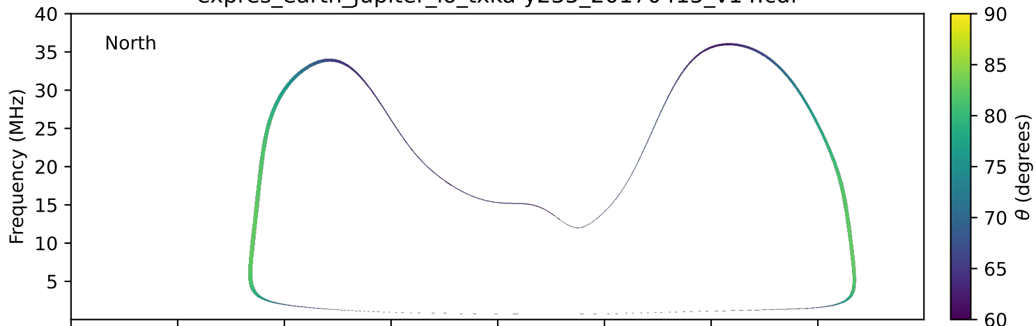
expres_earth_jupiter_io_txka-y235_20170415_v14.cdf
