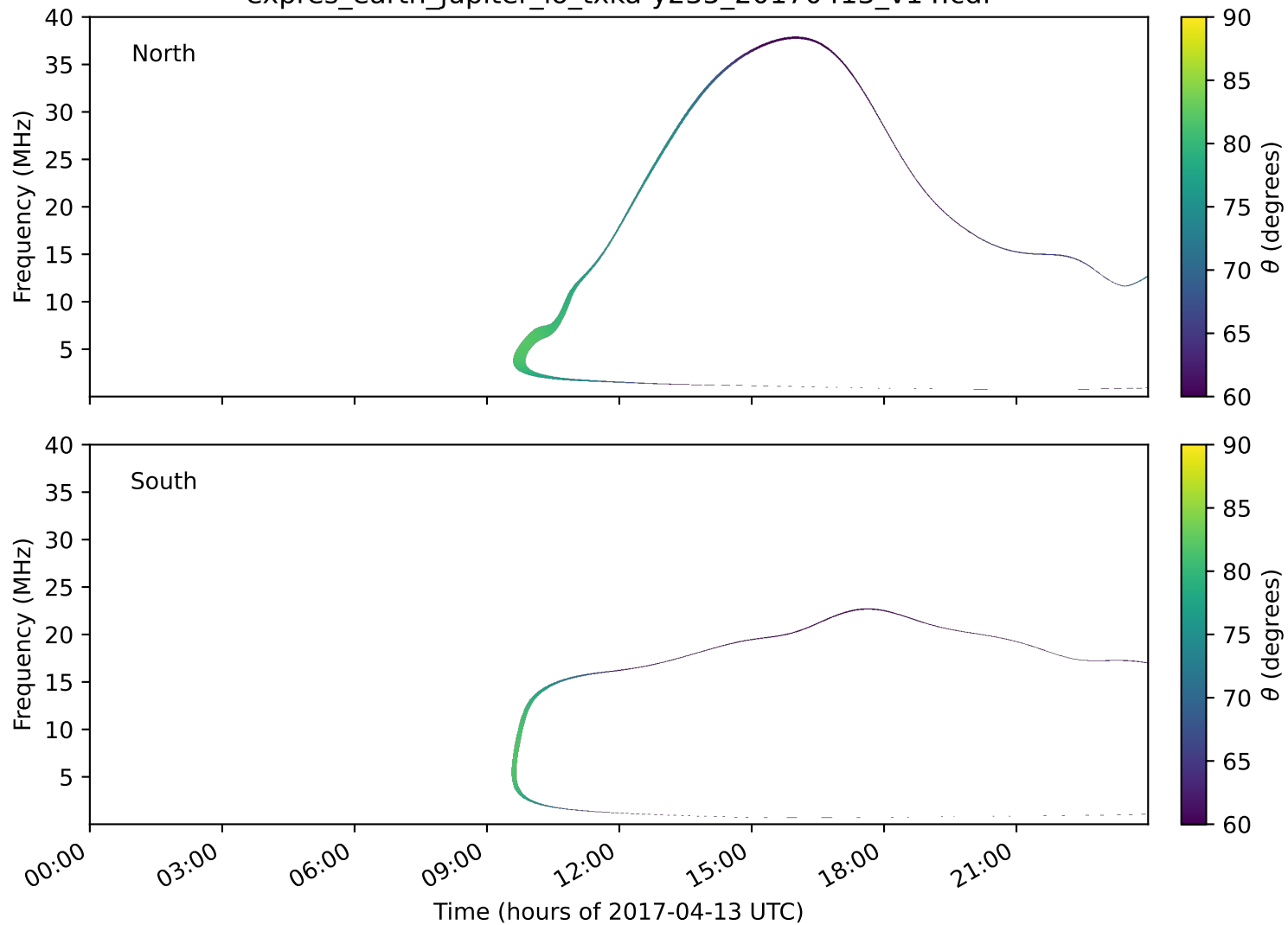
expres_earth_jupiter_io_txka-y235_20170413_v14.cdf
