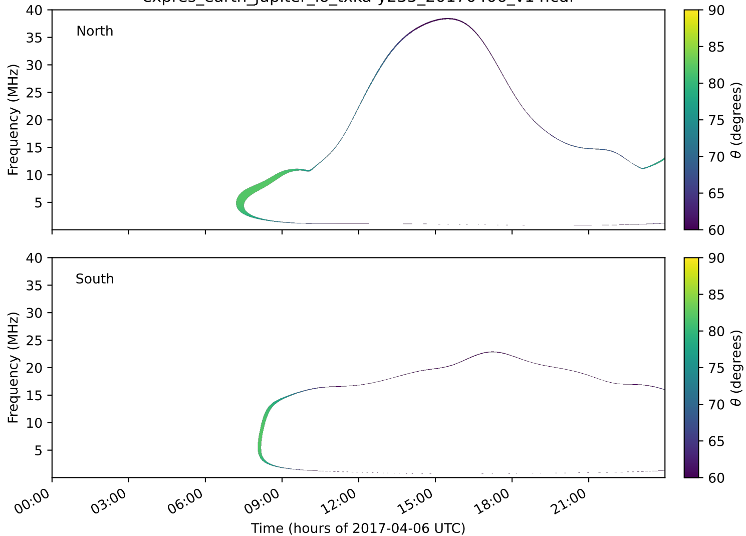
expres_earth_jupiter_io_txka-y235_20170406_v14.cdf
