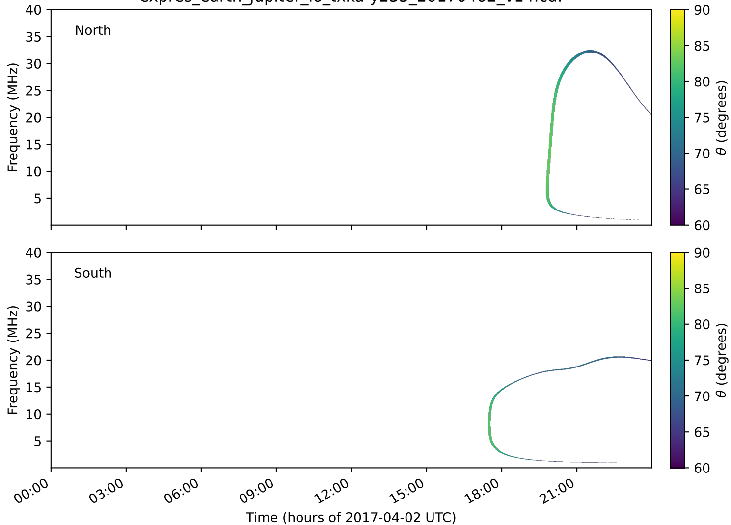
expres_earth_jupiter_io_txka-y235_20170402_v14.cdf
