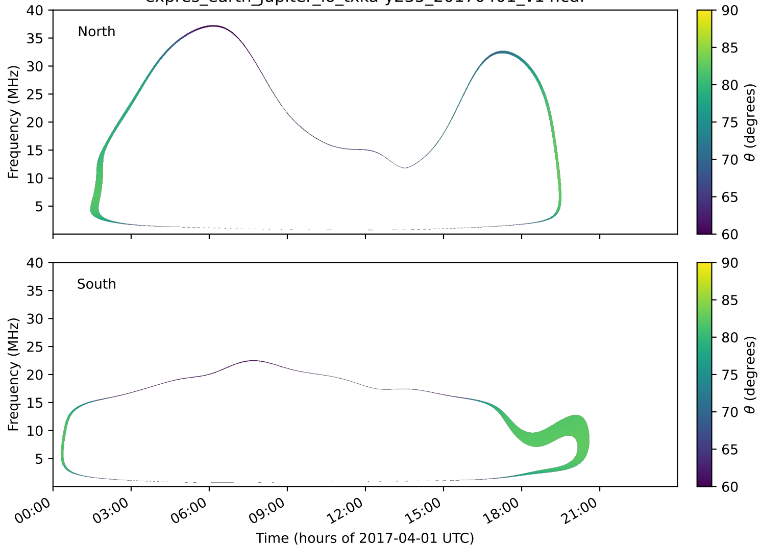
expres_earth_jupiter_io_txka-y235_20170401_v14.cdf
