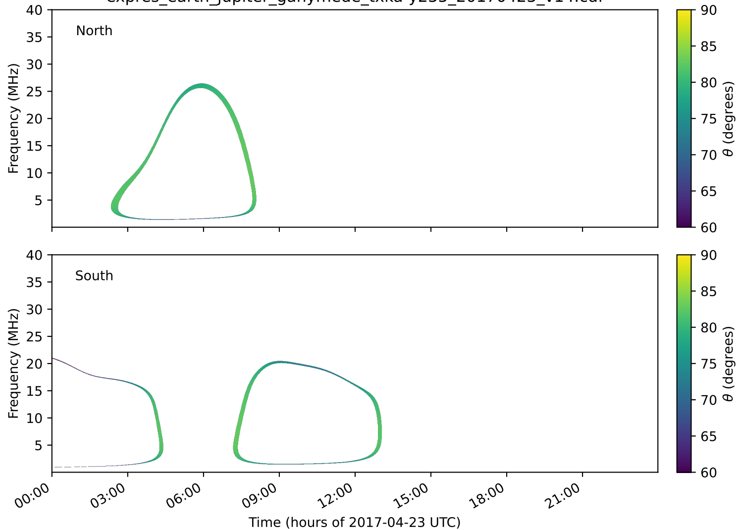
expres_earth_jupiter_ganymede_txka-y235_20170423_v14.cdf
