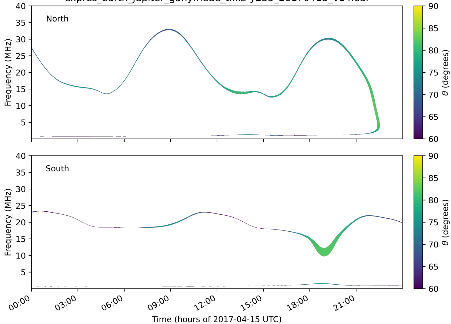
expres_earth_jupiter_ganymede_txka-y235_20170415_v14.cdf
