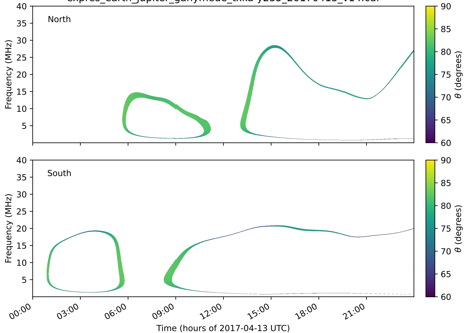
expres_earth_jupiter_ganymede_txka-y235_20170413_v14.cdf
