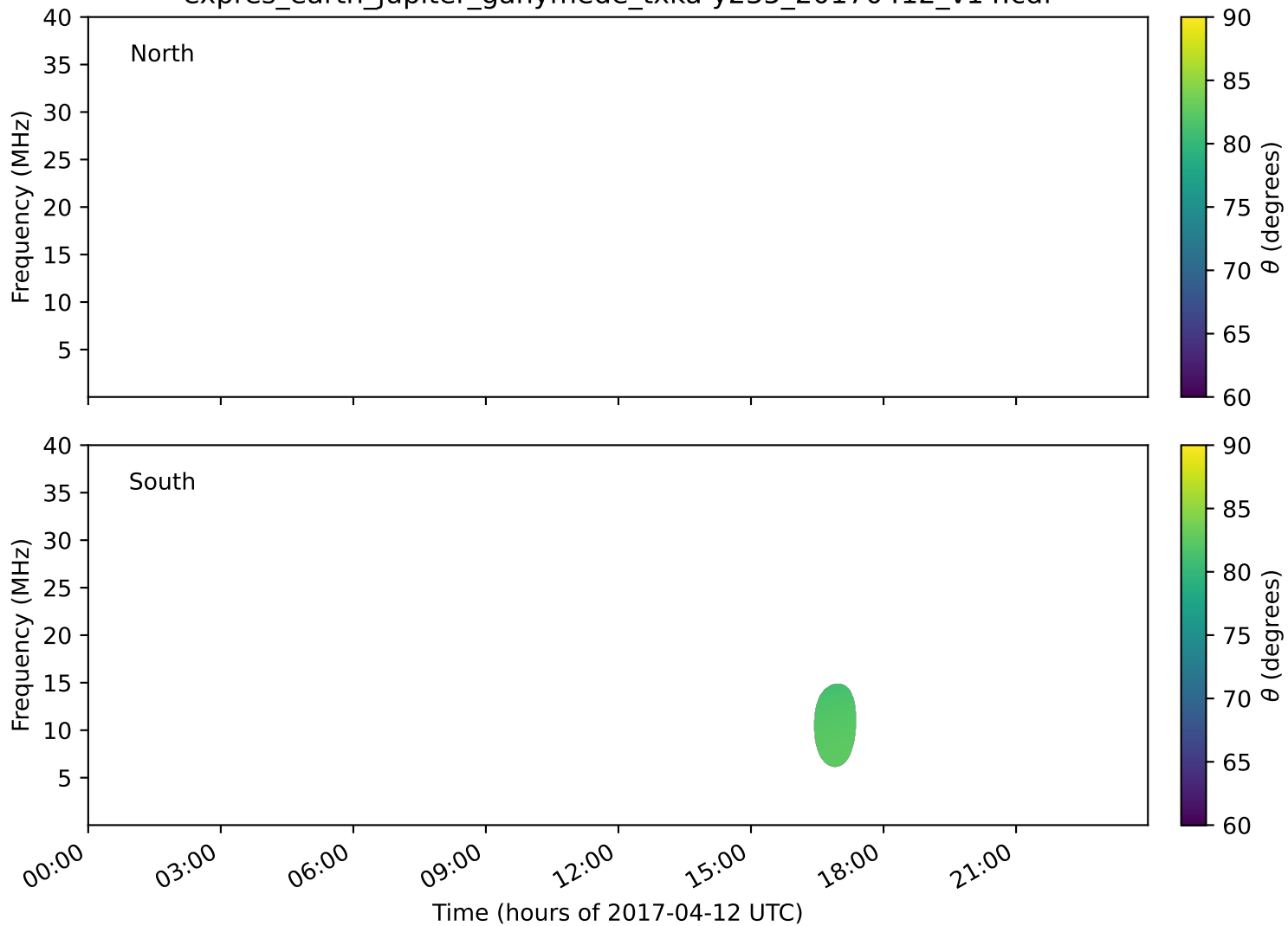
expres_earth_jupiter_ganymede_txka-y235_20170412_v14.cdf
