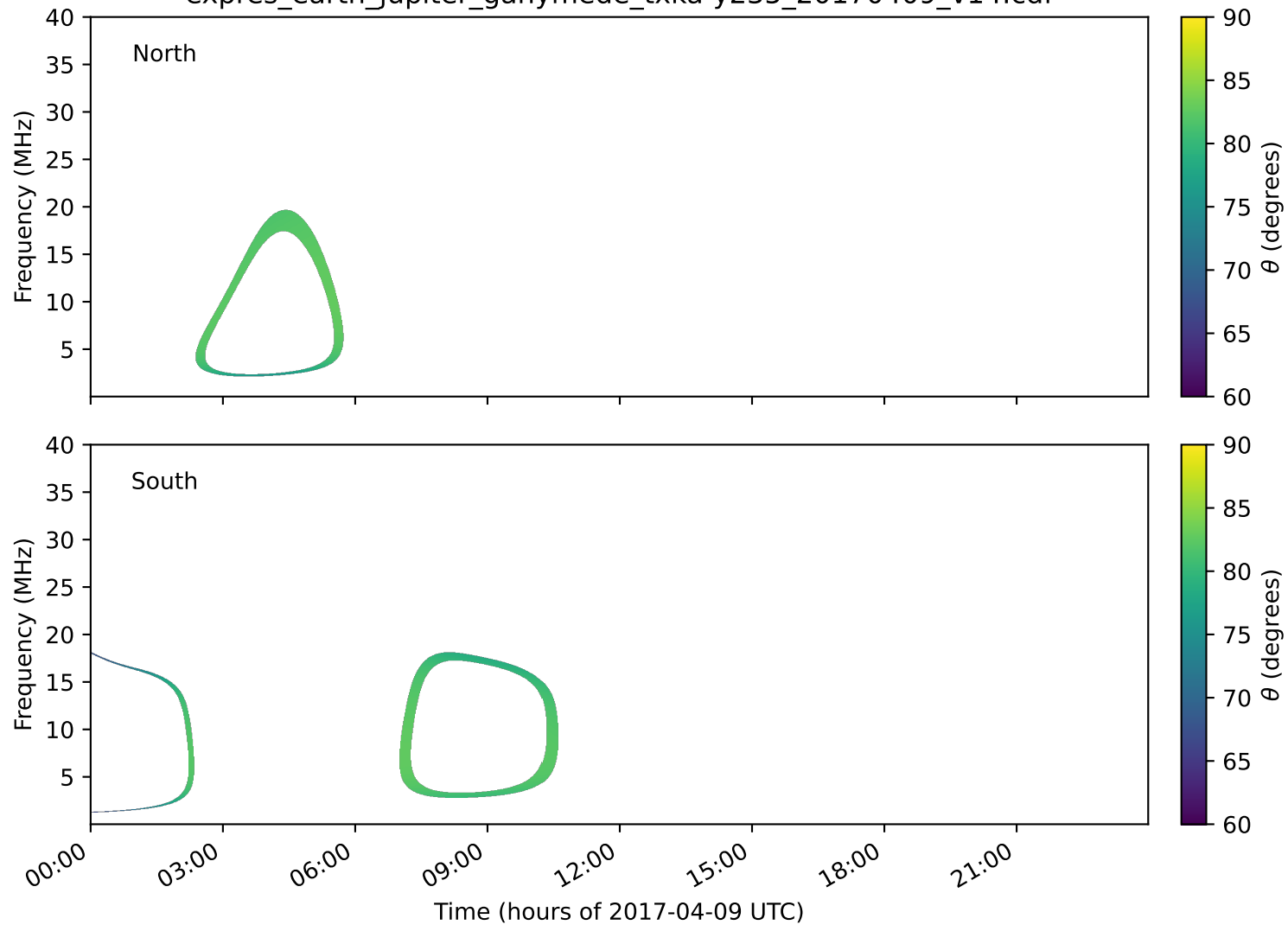
expres_earth_jupiter_ganymede_txka-y235_20170409_v14.cdf
