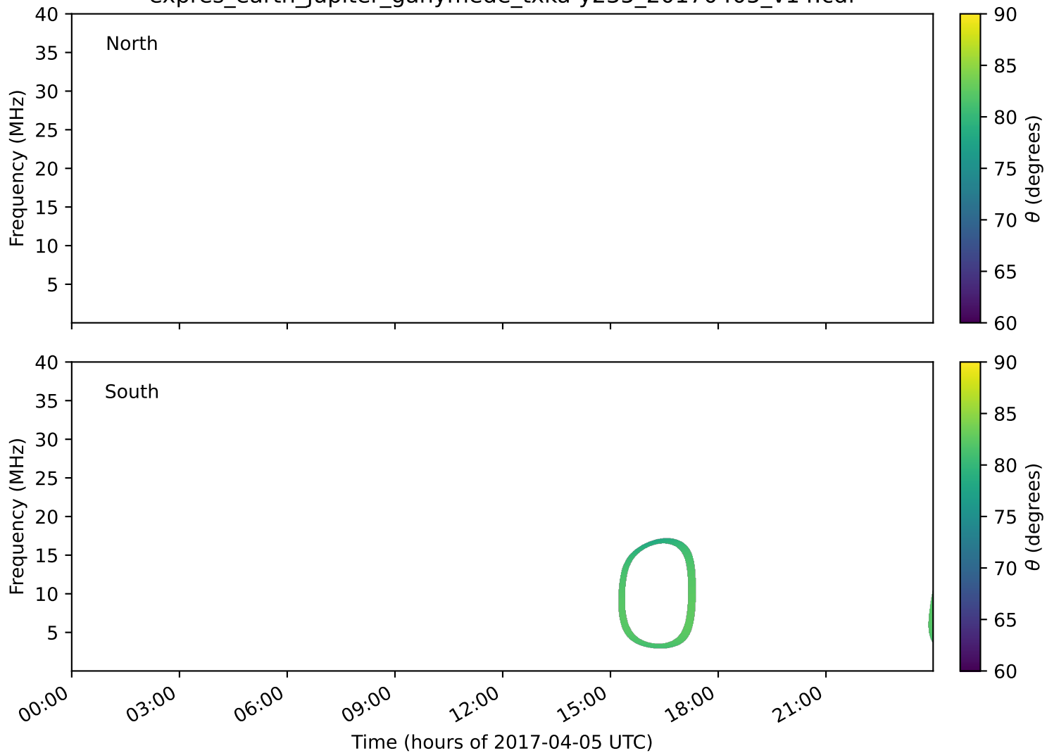
expres_earth_jupiter_ganymede_txka-y235_20170405_v14.cdf
