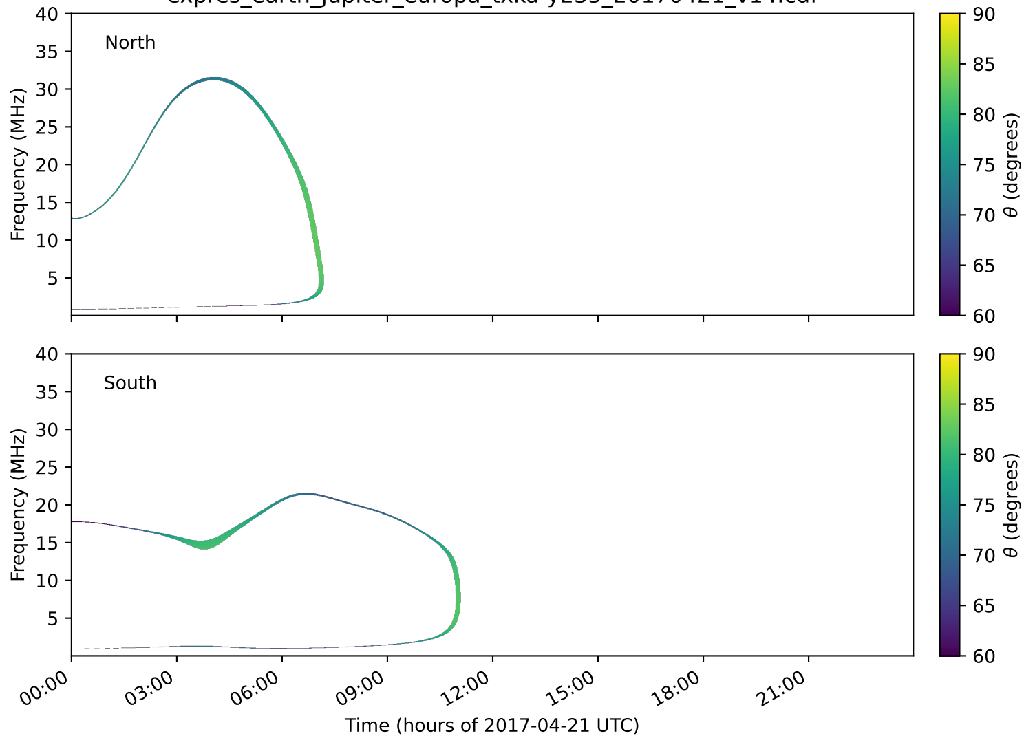
expres_earth_jupiter_europa_txka-y235_20170421_v14.cdf
