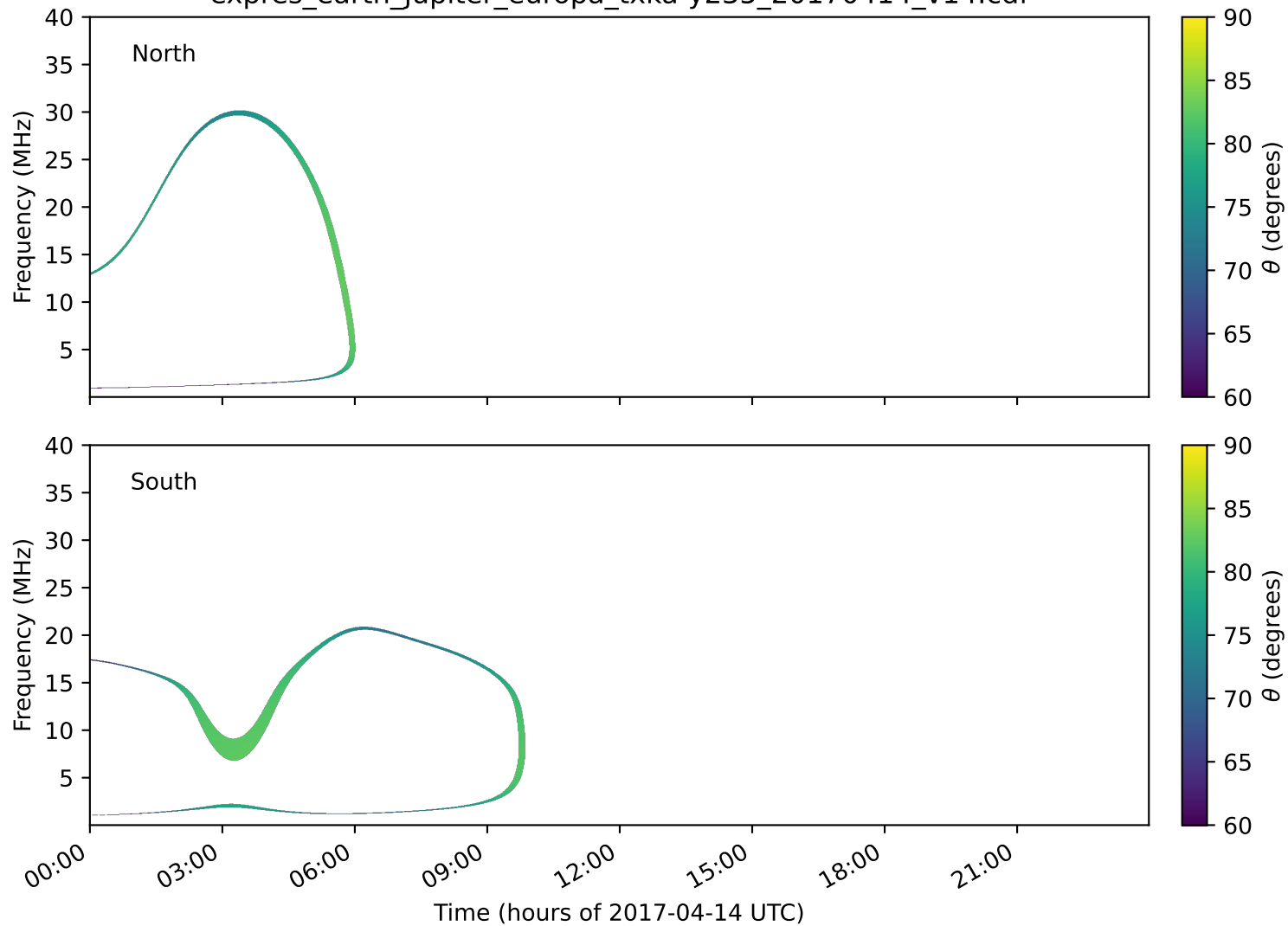
expres_earth_jupiter_europa_txka-y235_20170414_v14.cdf
