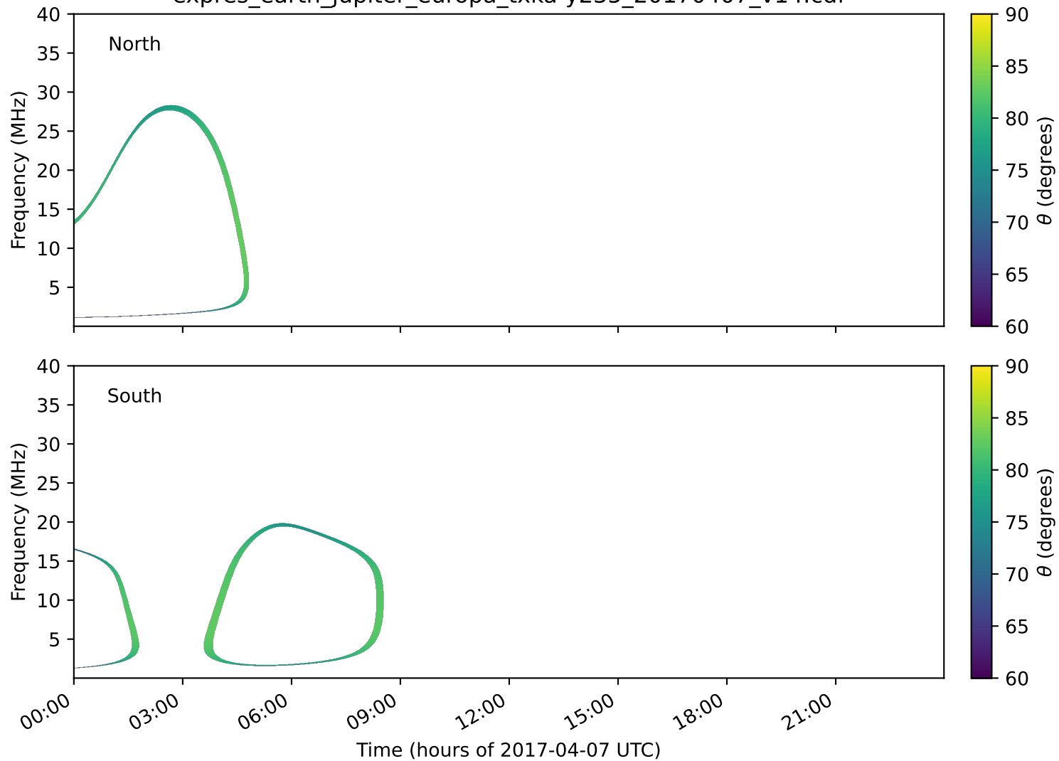
expres_earth_jupiter_europa_txka-y235_20170407_v14.cdf
