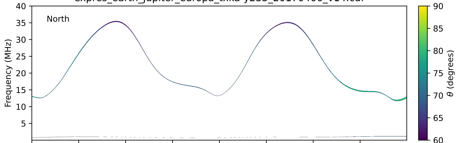
expres_earth_jupiter_europa_txka-y235_20170406_v14.cdf
