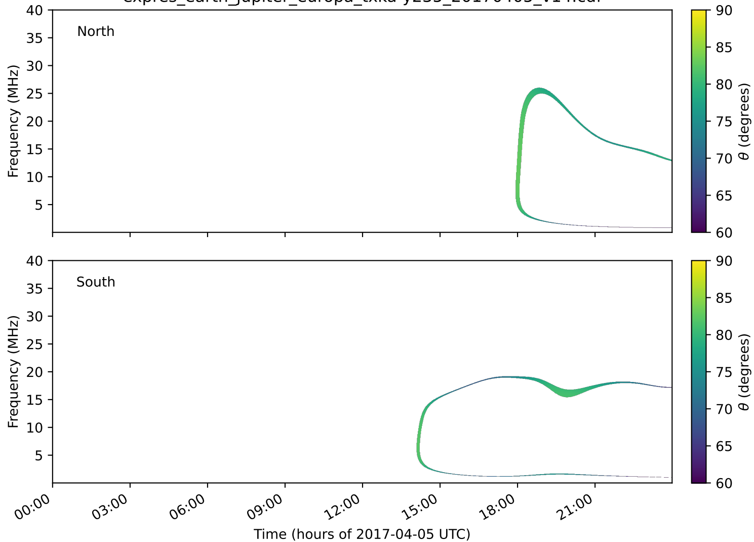
expres_earth_jupiter_europa_txka-y235_20170405_v14.cdf
