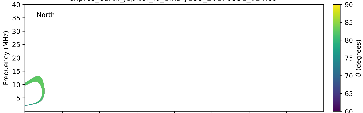
expres_earth_jupiter_io_txka-y235_20170331_v14.cdf
