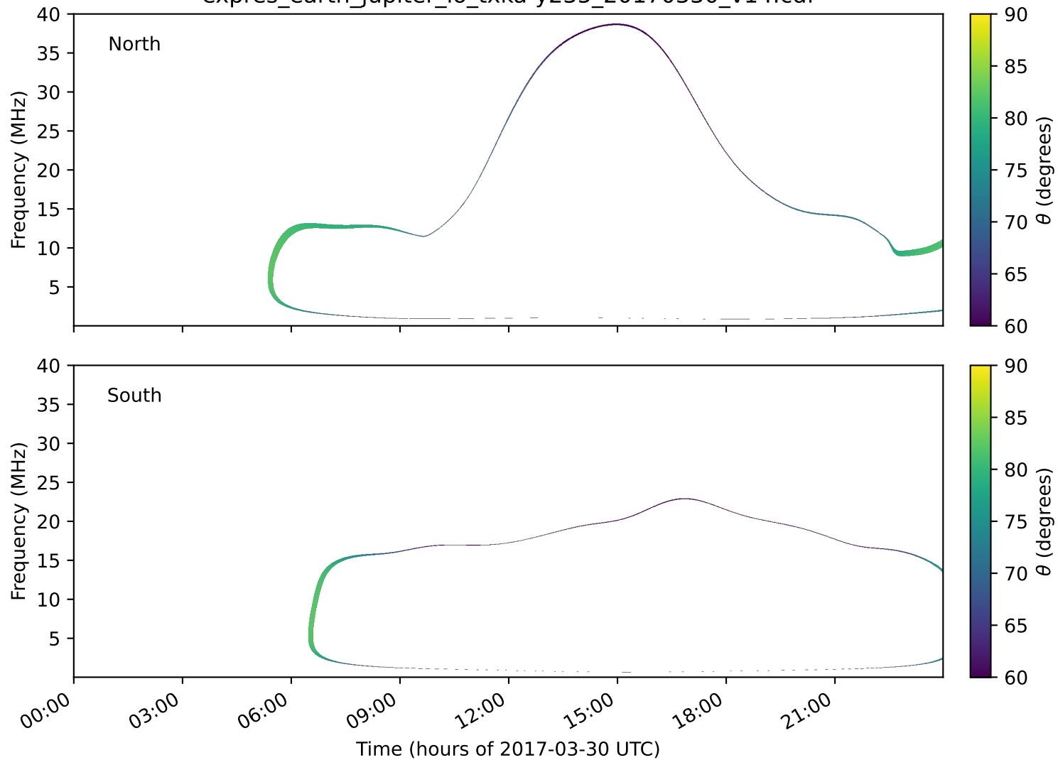
expres_earth_jupiter_io_txka-y235_20170330_v14.cdf
