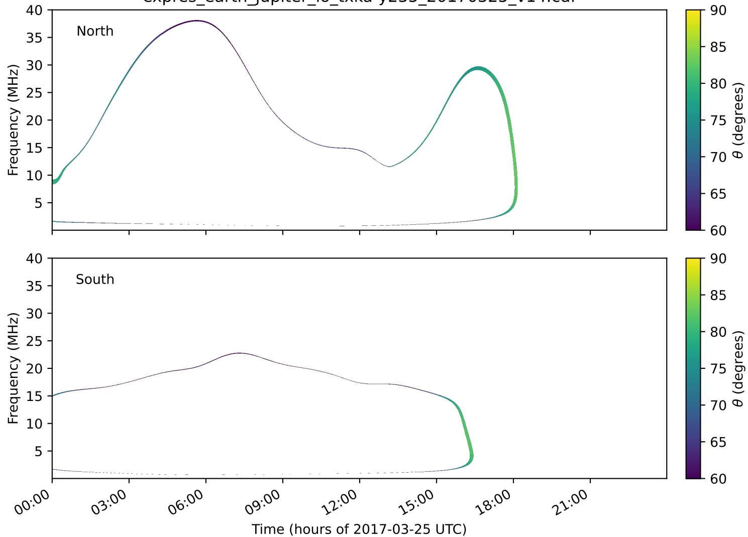
expres_earth_jupiter_io_txka-y235_20170325_v14.cdf
