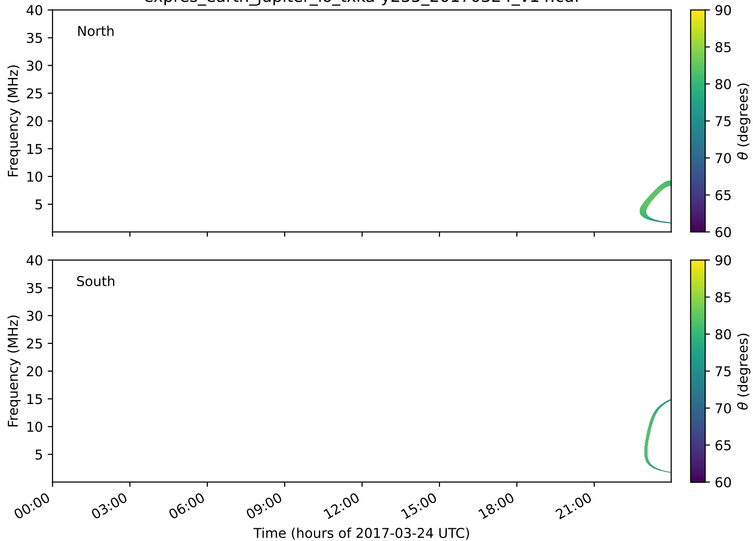
expres_earth_jupiter_io_txka-y235_20170324_v14.cdf
