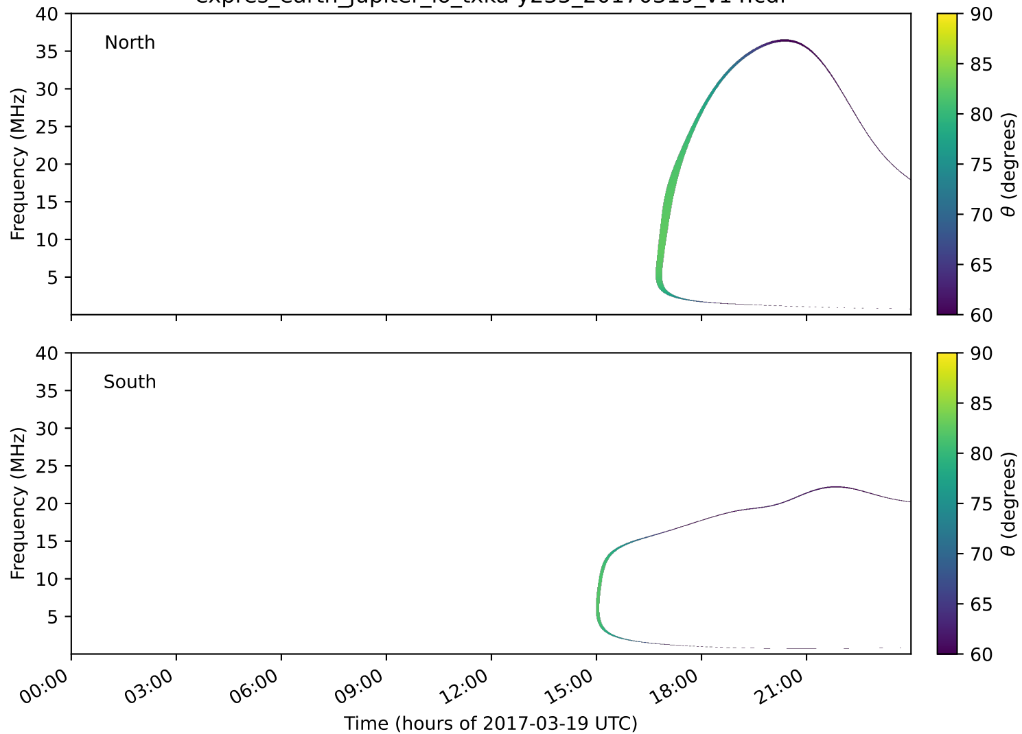
expres_earth_jupiter_io_txka-y235_20170319_v14.cdf
