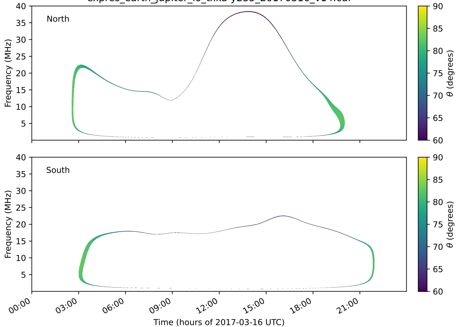
expres_earth_jupiter_io_txka-y235_20170316_v14.cdf
