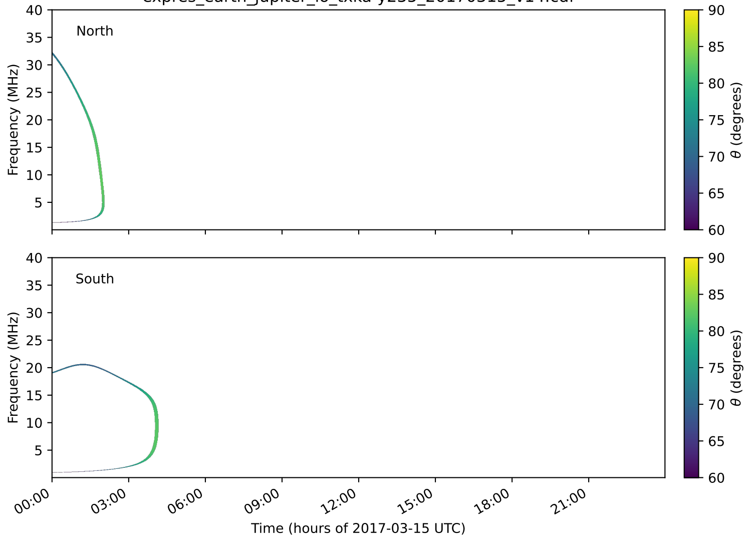
expres_earth_jupiter_io_txka-y235_20170315_v14.cdf
