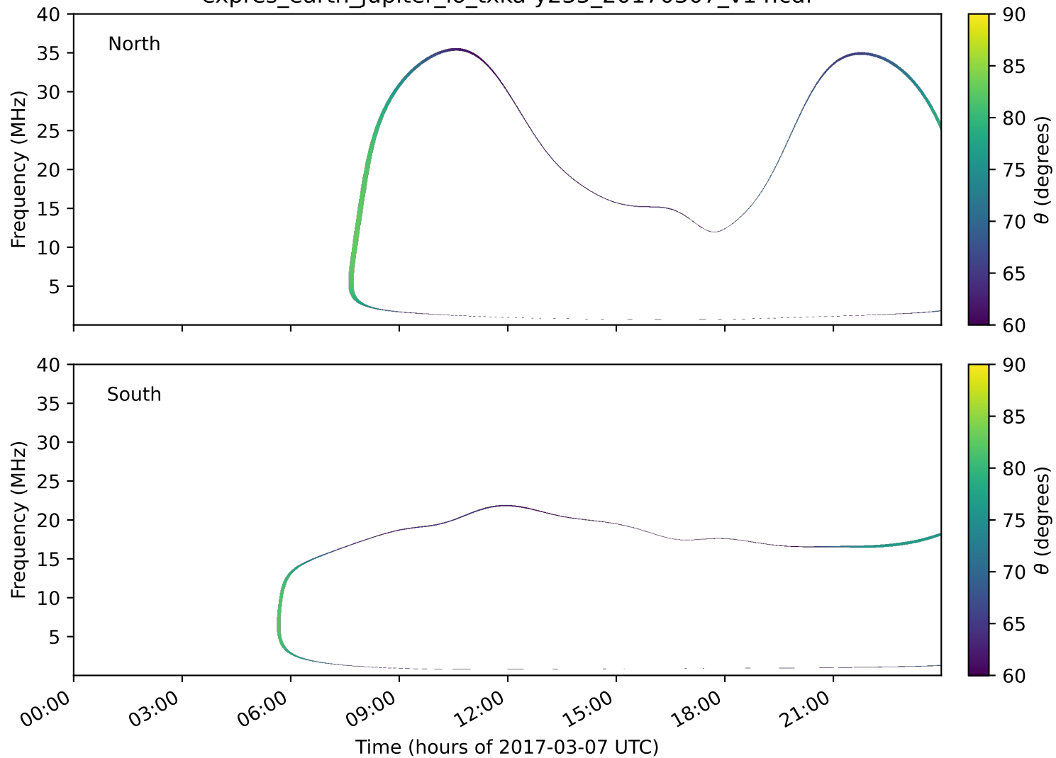
expres_earth_jupiter_io_txka-y235_20170307_v14.cdf
