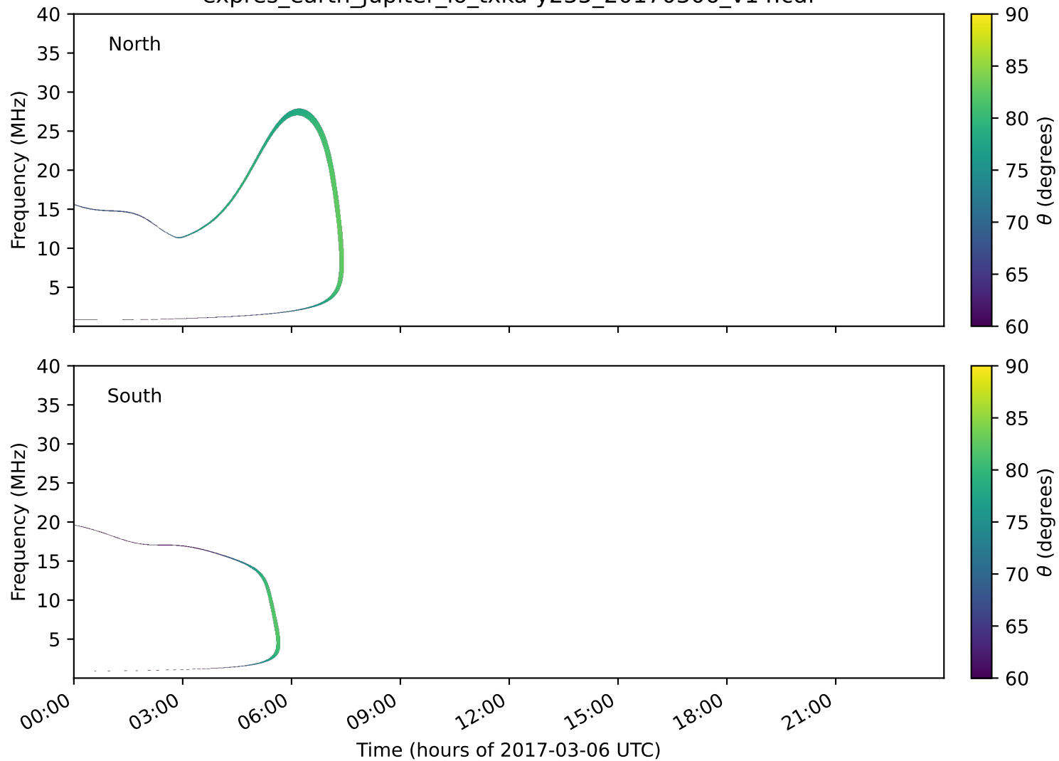
expres_earth_jupiter_io_txka-y235_20170306_v14.cdf
