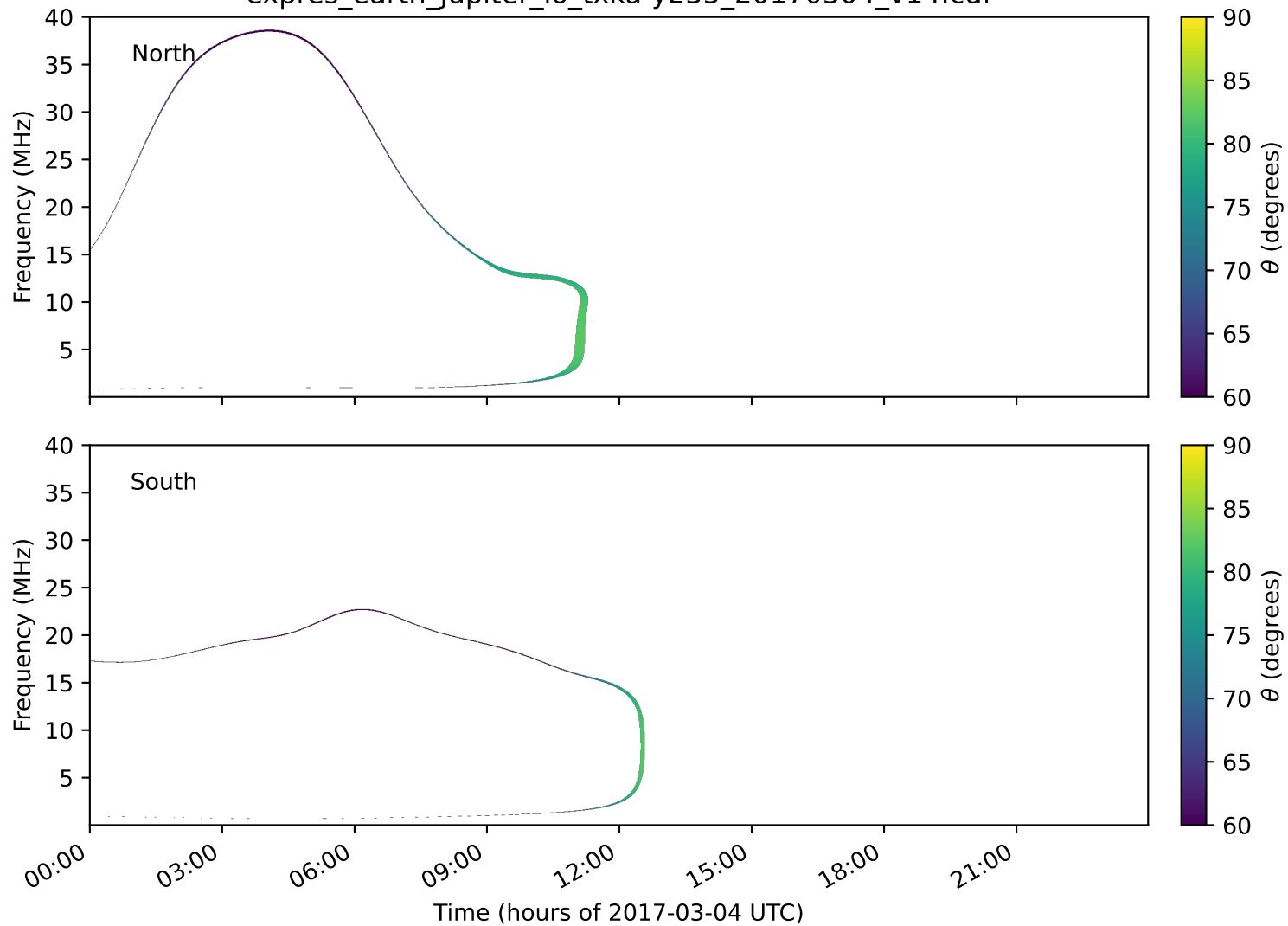
expres_earth_jupiter_io_txka-y235_20170304_v14.cdf
