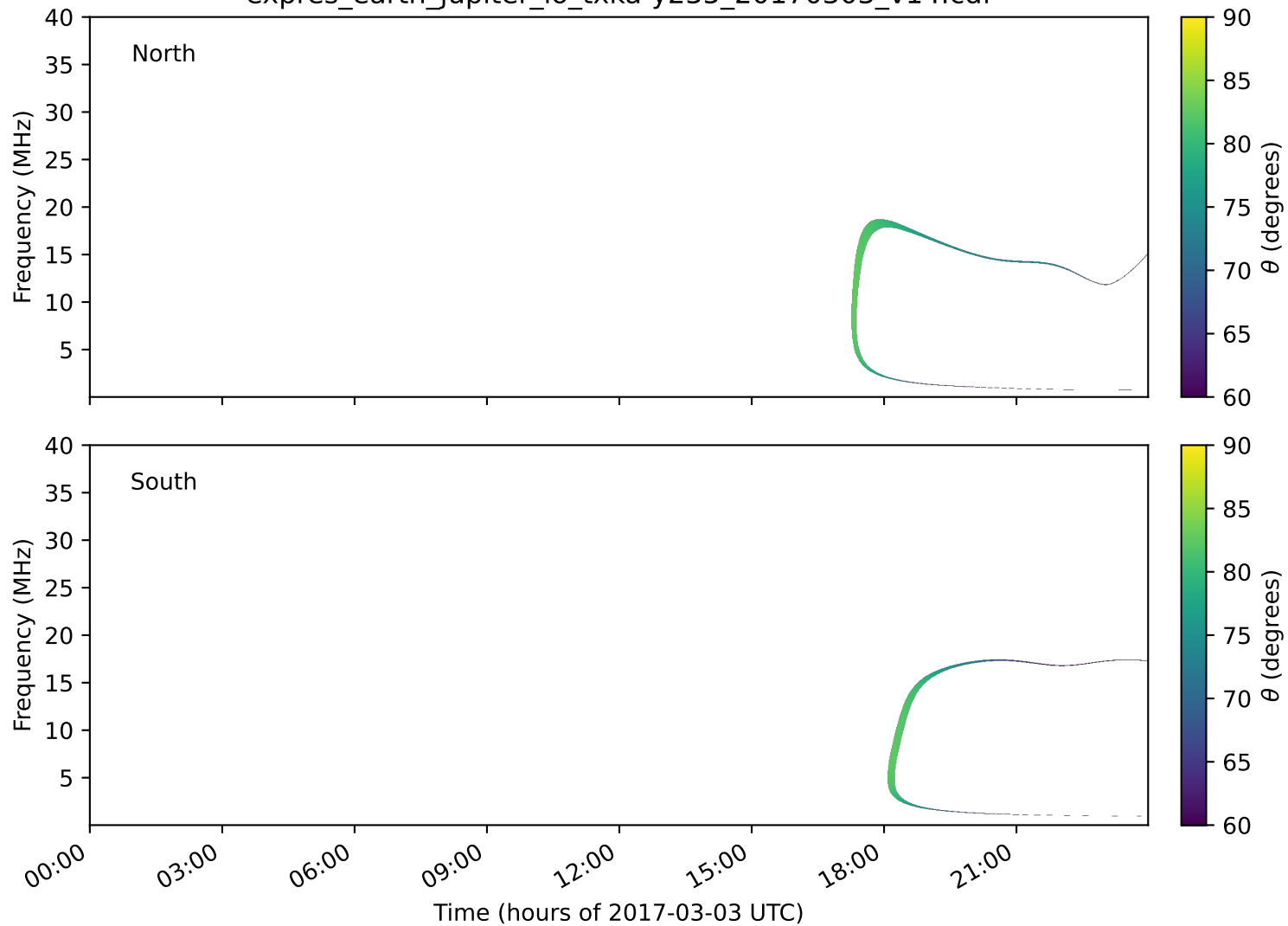
expres_earth_jupiter_io_txka-y235_20170303_v14.cdf
