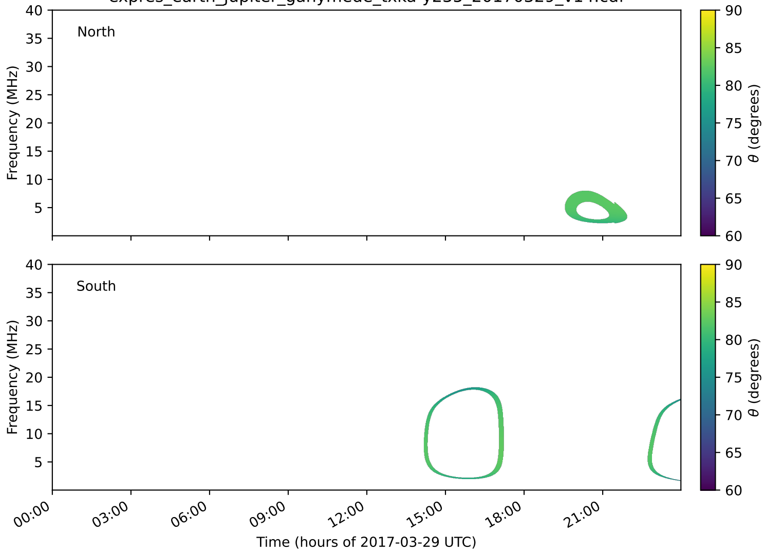
expres_earth_jupiter_ganymede_txka-y235_20170329_v14.cdf
