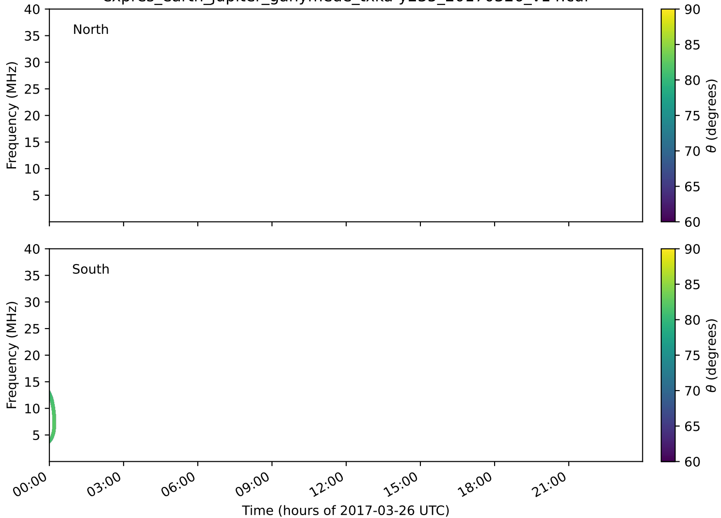
expres_earth_jupiter_ganymede_txka-y235_20170326_v14.cdf
