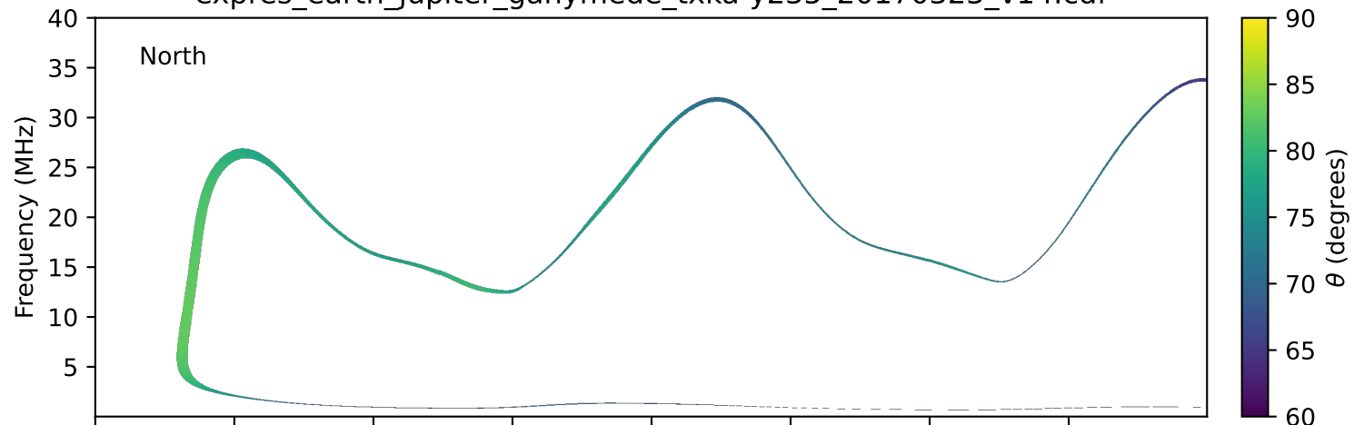
expres_earth_jupiter_ganymede_txka-y235_20170323_v14.cdf
