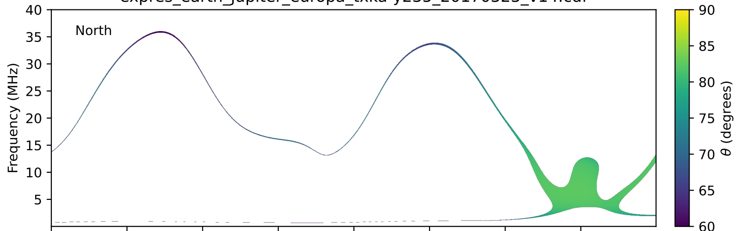
expres_earth_jupiter_europa_txka-y235_20170323_v14.cdf
