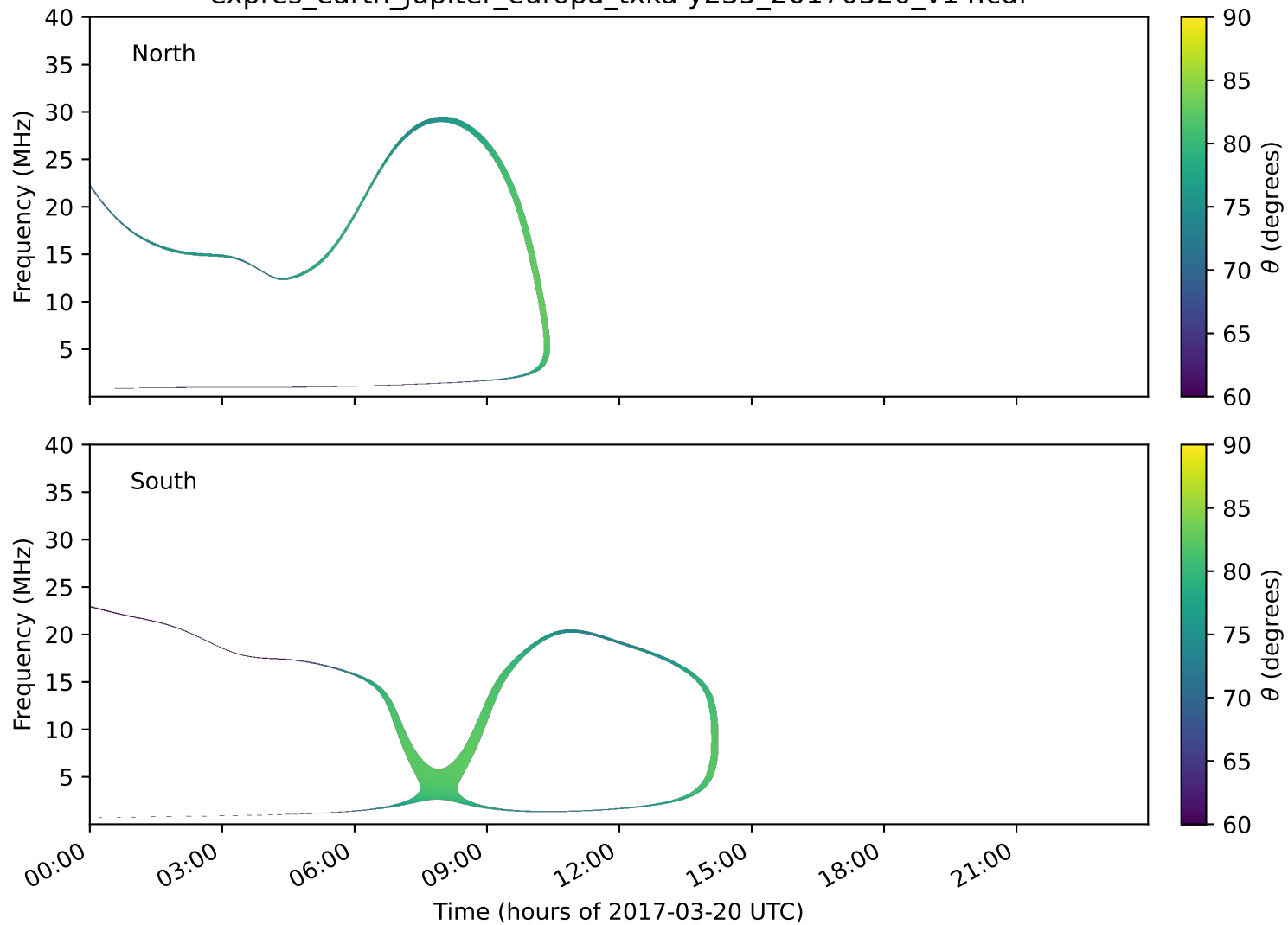
expres_earth_jupiter_europa_txka-y235_20170320_v14.cdf
