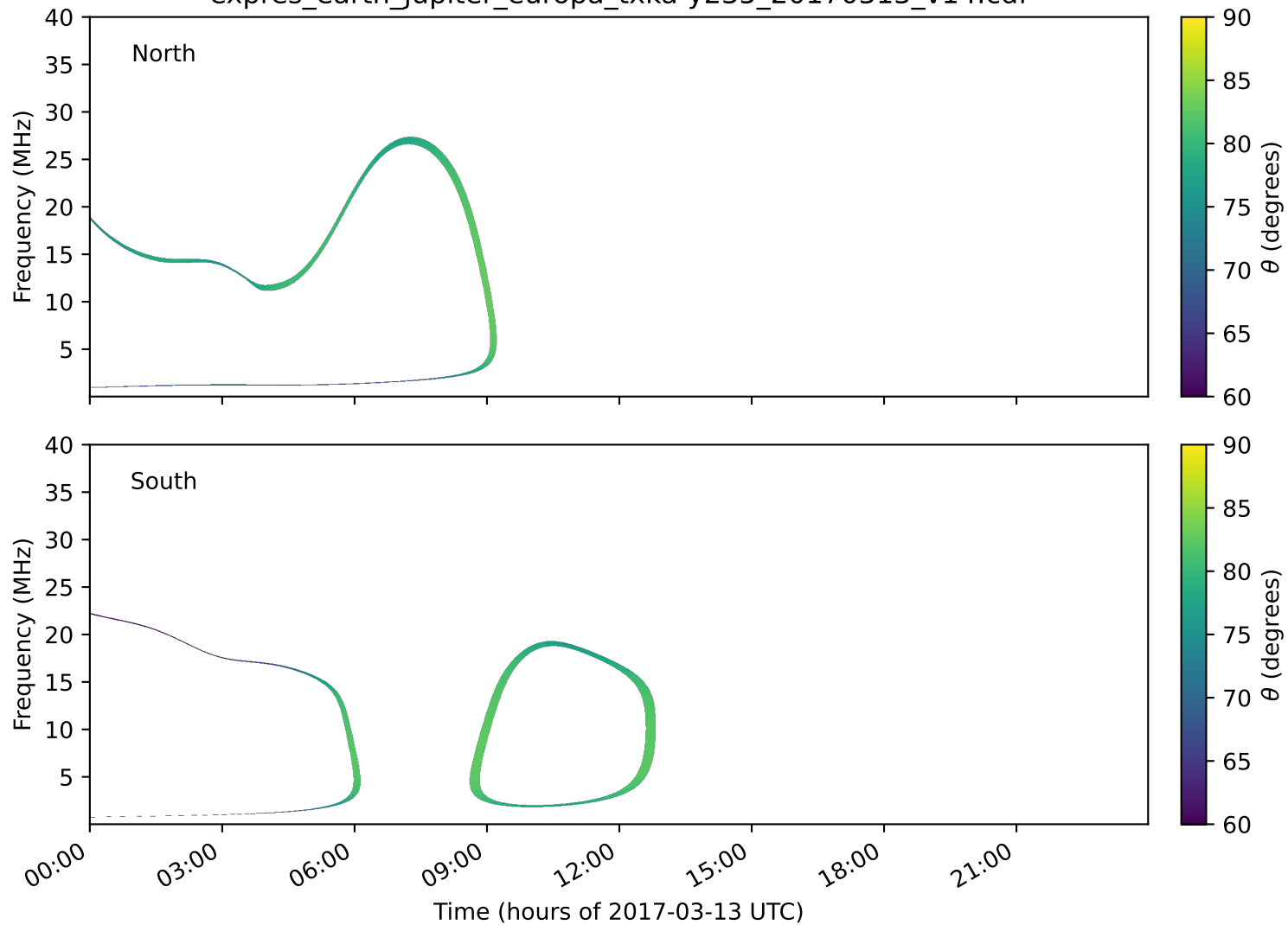
expres_earth_jupiter_europa_txka-y235_20170313_v14.cdf
