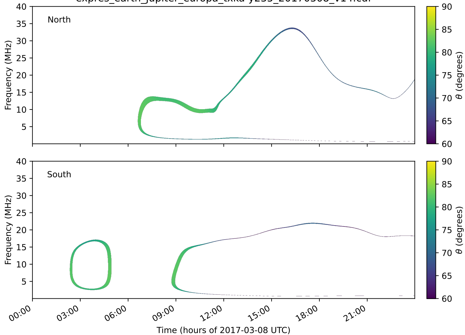
expres_earth_jupiter_europa_txka-y235_20170308_v14.cdf
