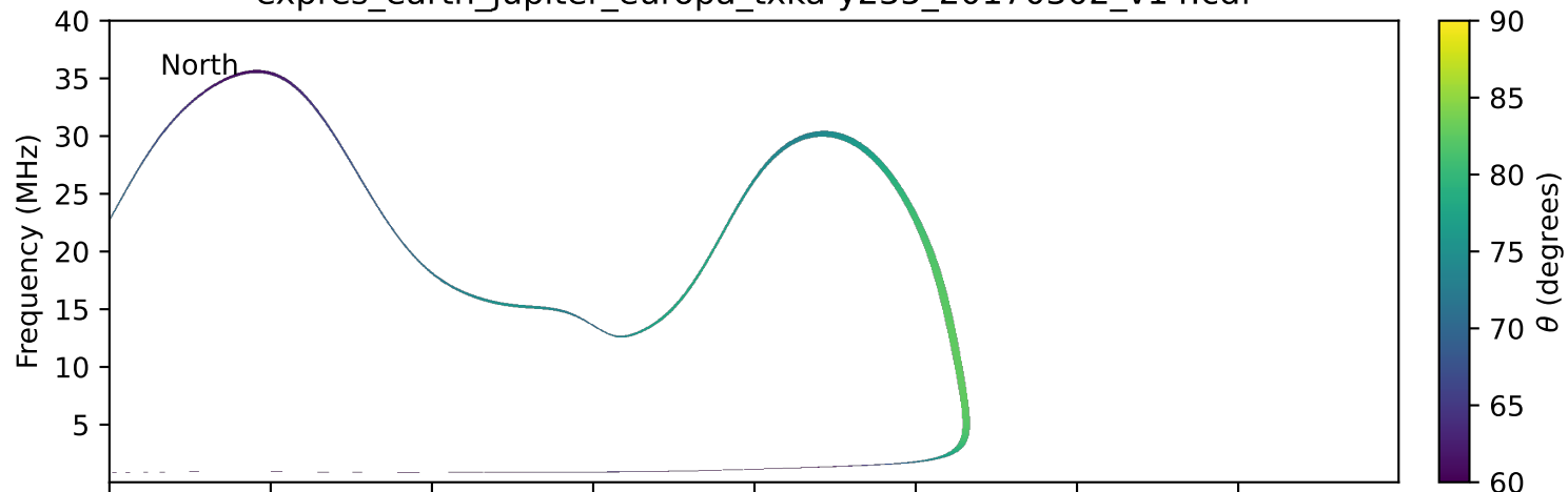
expres_earth_jupiter_europa_txka-y235_20170302_v14.cdf
