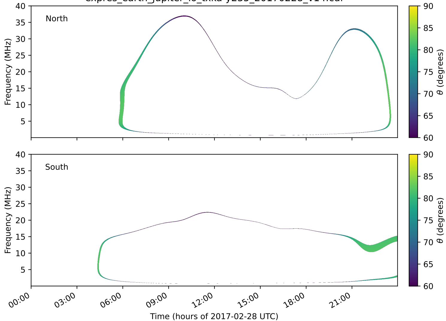
expres_earth_jupiter_io_txka-y235_20170228_v14.cdf
